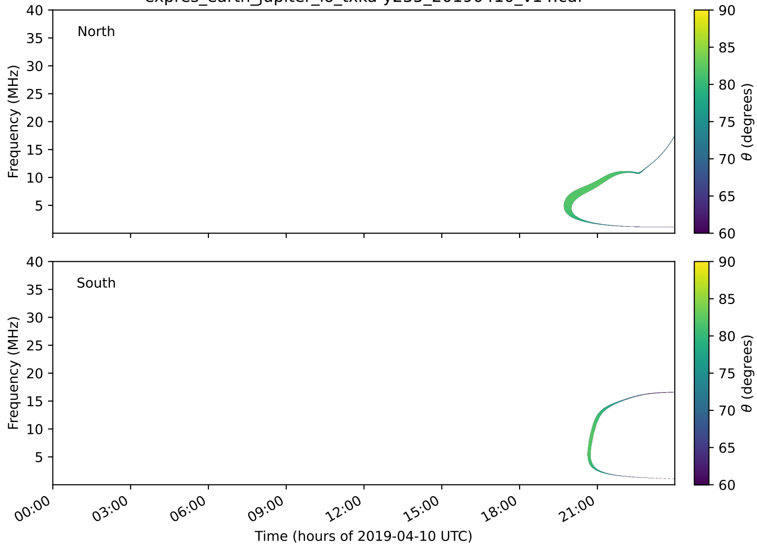
expres_earth_jupiter_io_txka-y235_20190410_v14.cdf
