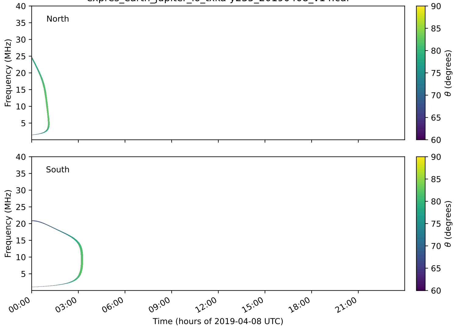
expres_earth_jupiter_io_txka-y235_20190408_v14.cdf
