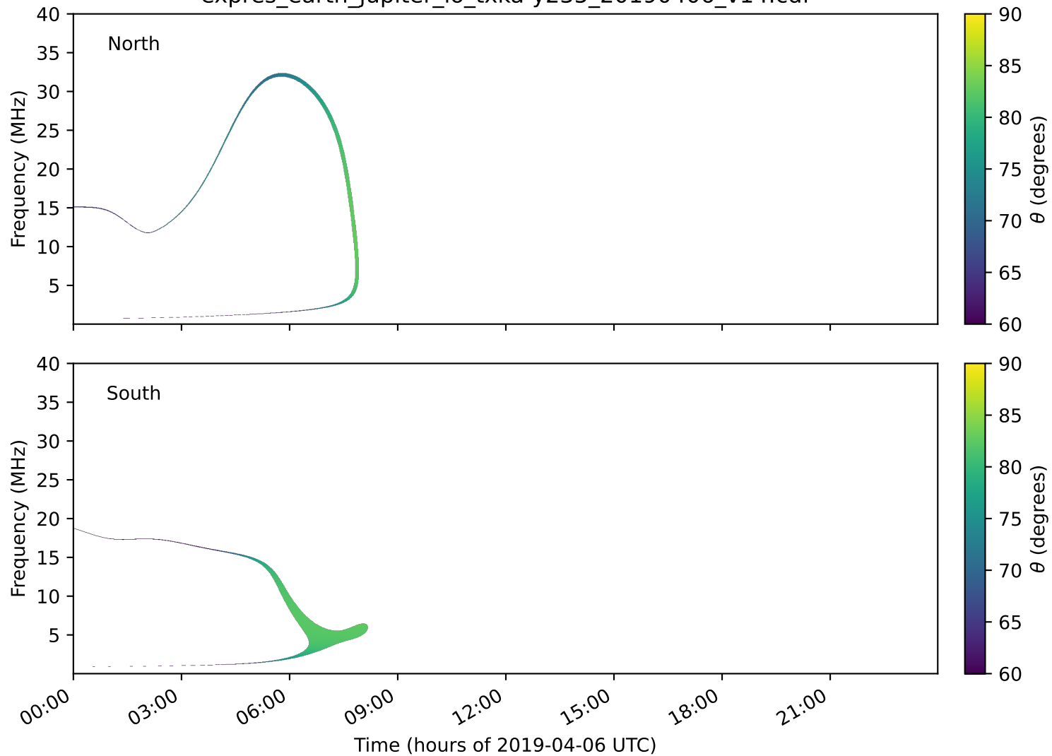
expres_earth_jupiter_io_txka-y235_20190406_v14.cdf
