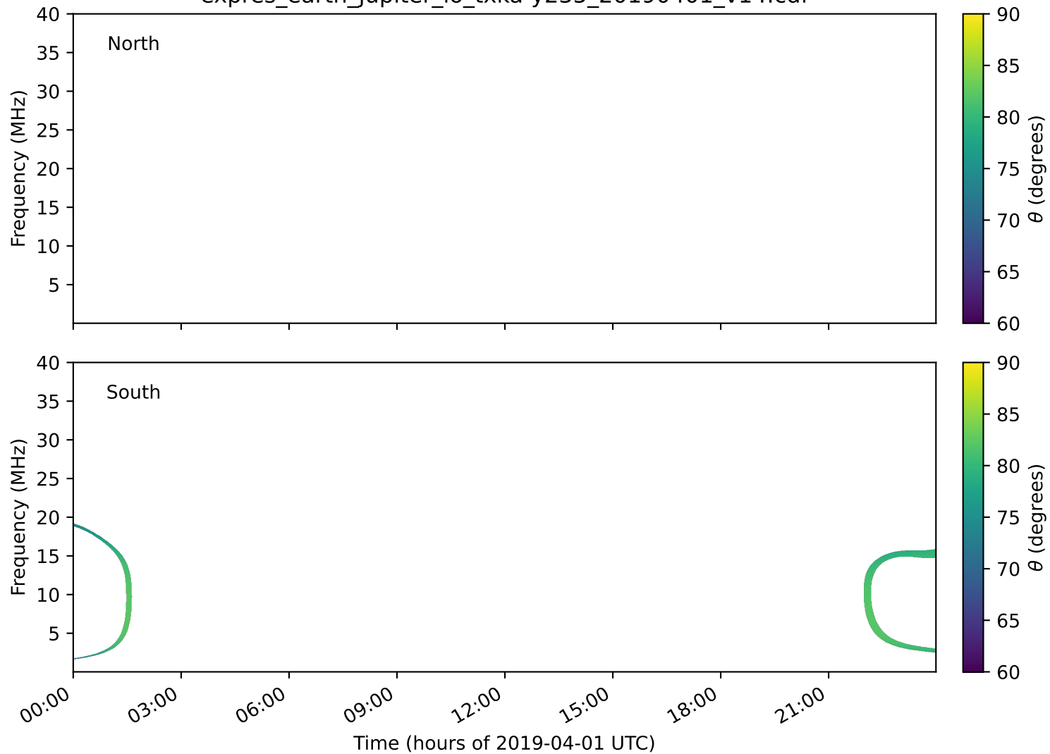
expres_earth_jupiter_io_txka-y235_20190401_v14.cdf
