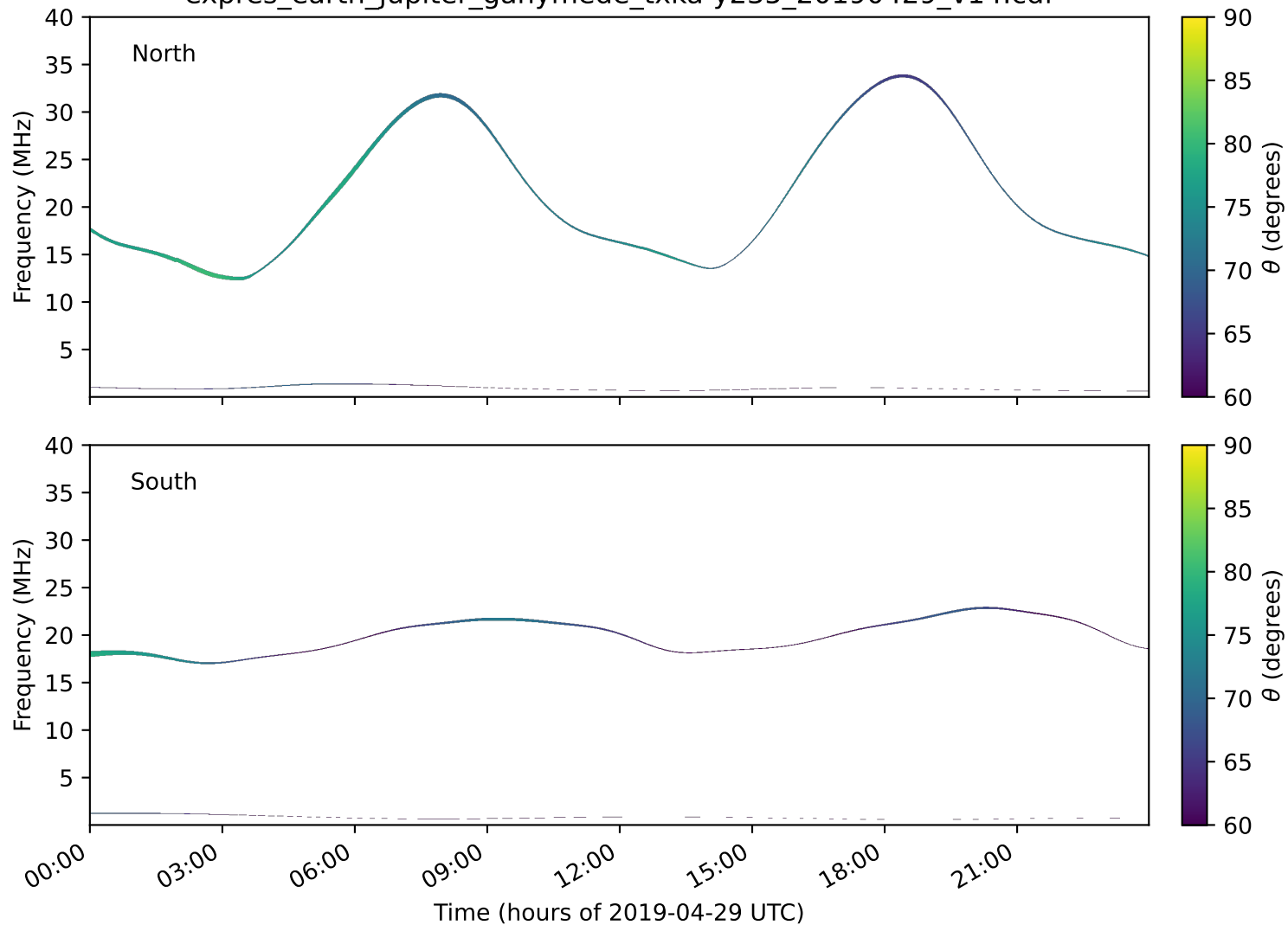
expres_earth_jupiter_ganymede_txka-y235_20190429_v14.cdf
