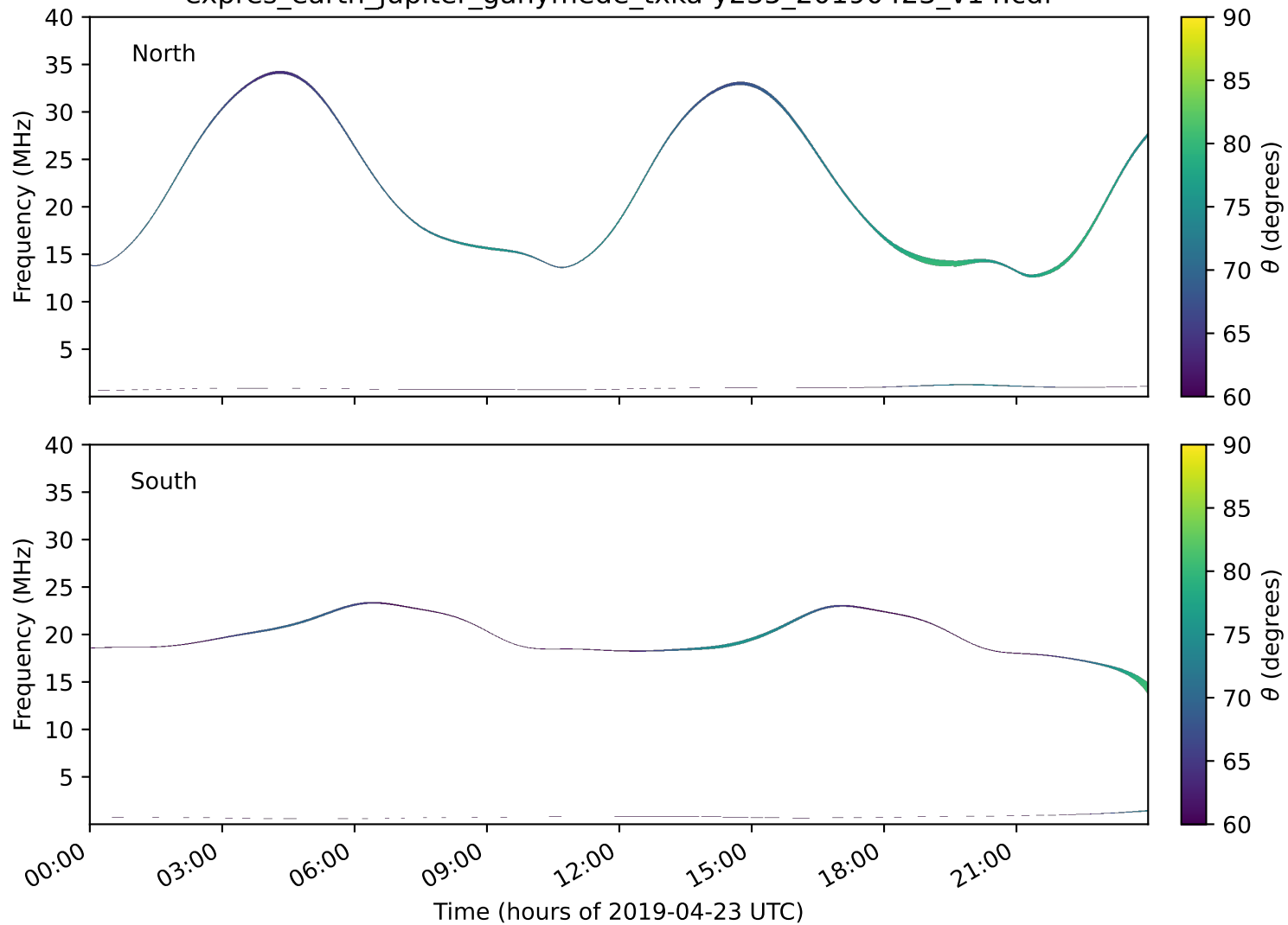
expres_earth_jupiter_ganymede_txka-y235_20190423_v14.cdf
