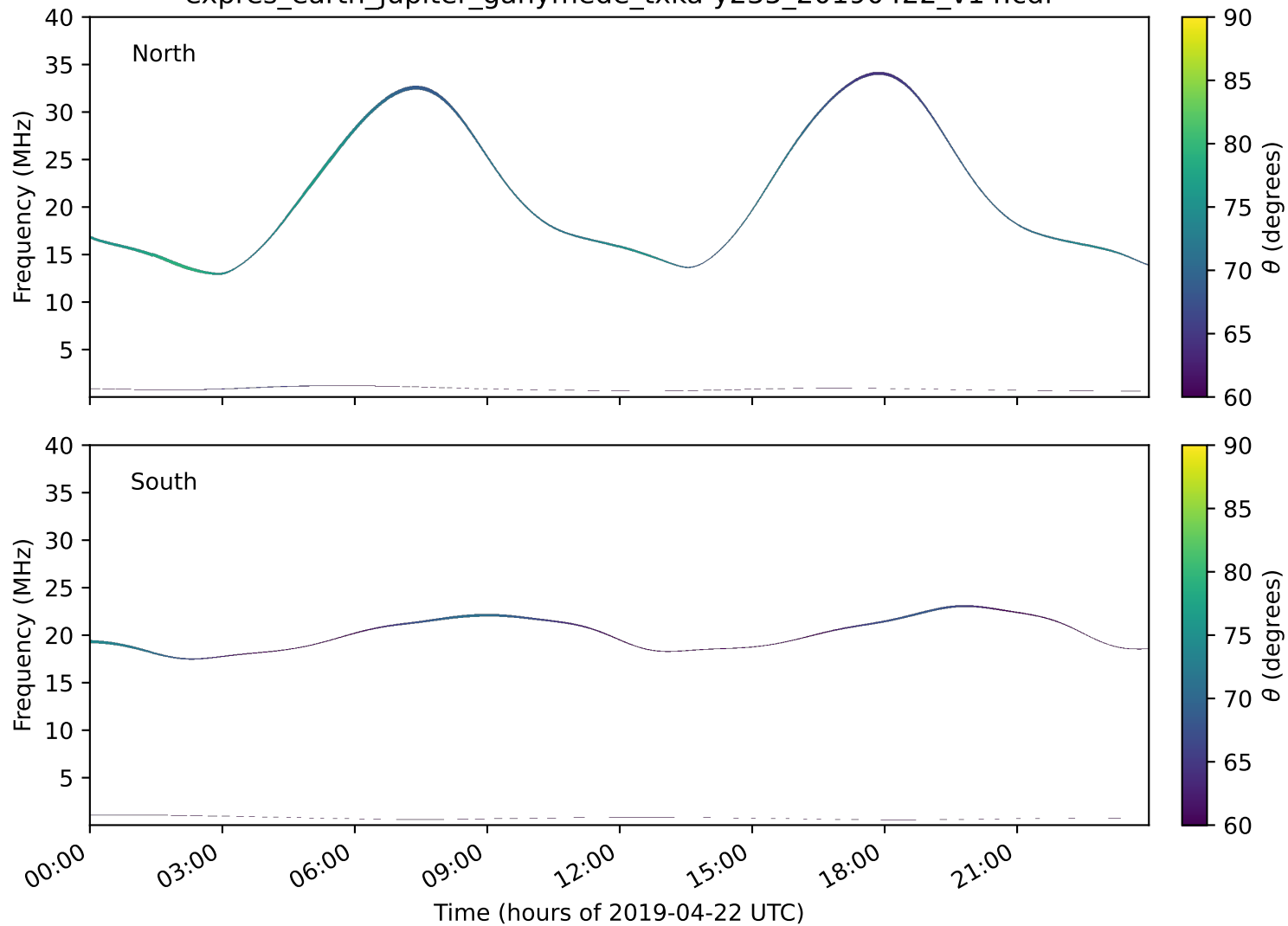
expres_earth_jupiter_ganymede_txka-y235_20190422_v14.cdf
