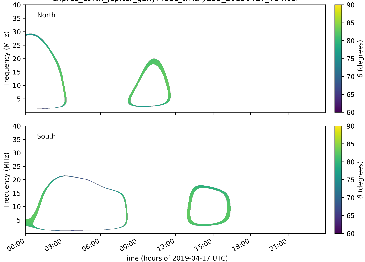
expres_earth_jupiter_ganymede_txka-y235_20190417_v14.cdf
