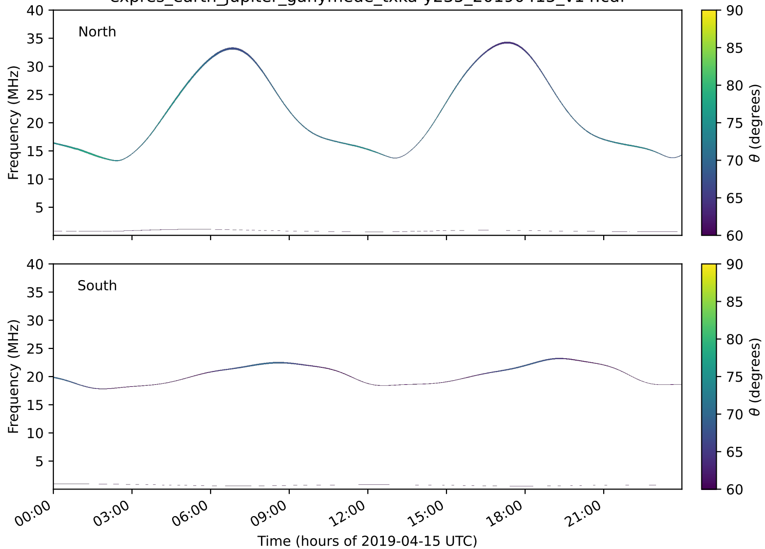
expres_earth_jupiter_ganymede_txka-y235_20190415_v14.cdf
