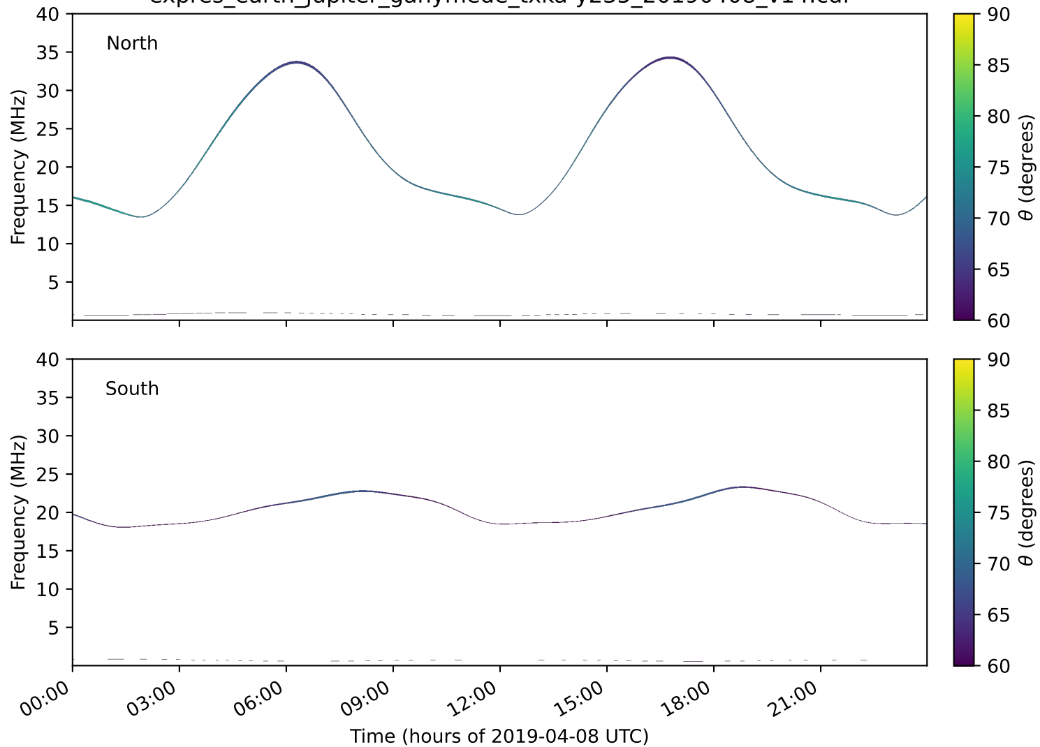
expres_earth_jupiter_ganymede_txka-y235_20190408_v14.cdf
