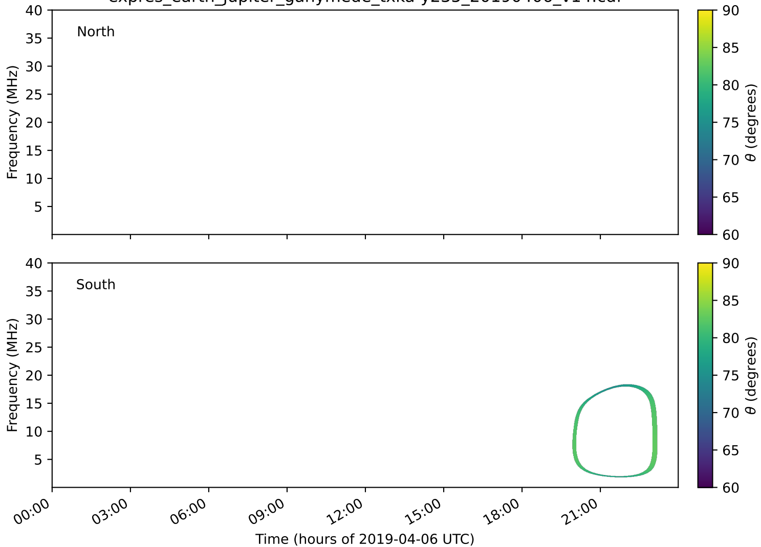
expres_earth_jupiter_ganymede_txka-y235_20190406_v14.cdf
