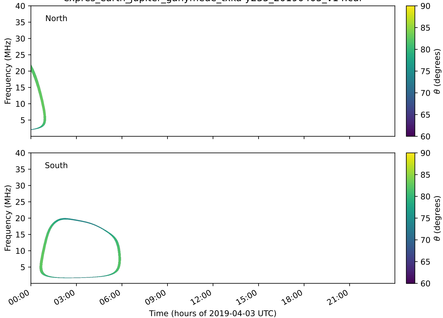
expres_earth_jupiter_ganymede_txka-y235_20190403_v14.cdf
