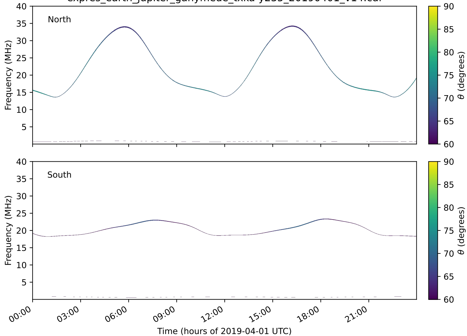
expres_earth_jupiter_ganymede_txka-y235_20190401_v14.cdf
