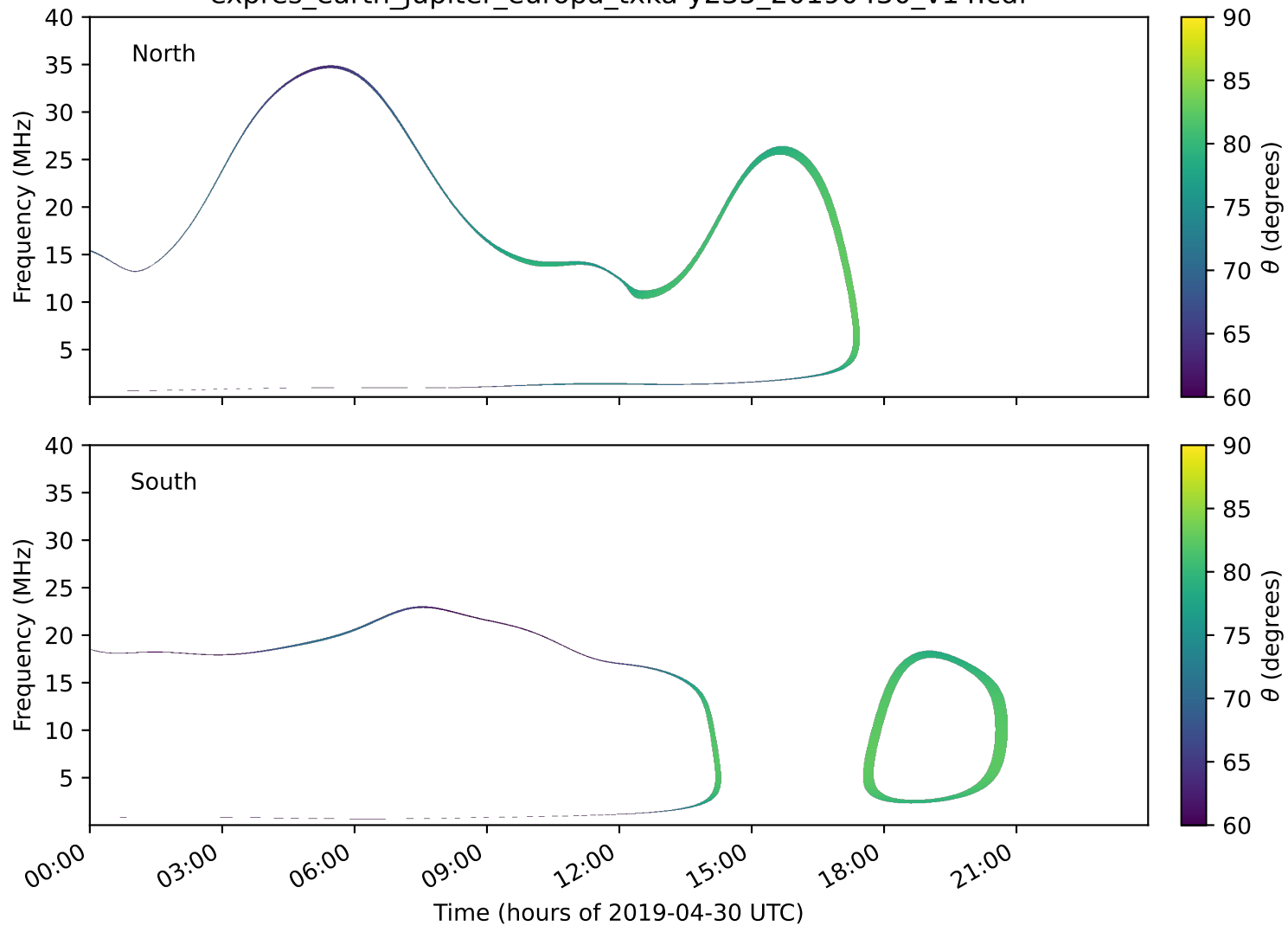
expres_earth_jupiter_europa_txka-y235_20190430_v14.cdf
