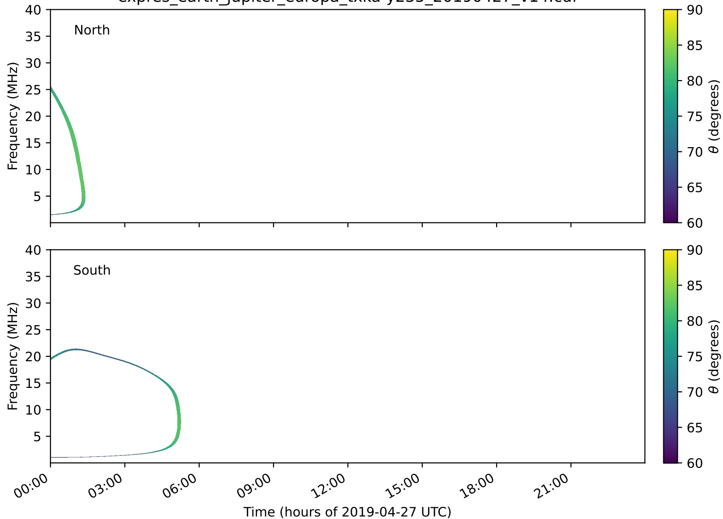
expres_earth_jupiter_europa_txka-y235_20190427_v14.cdf
