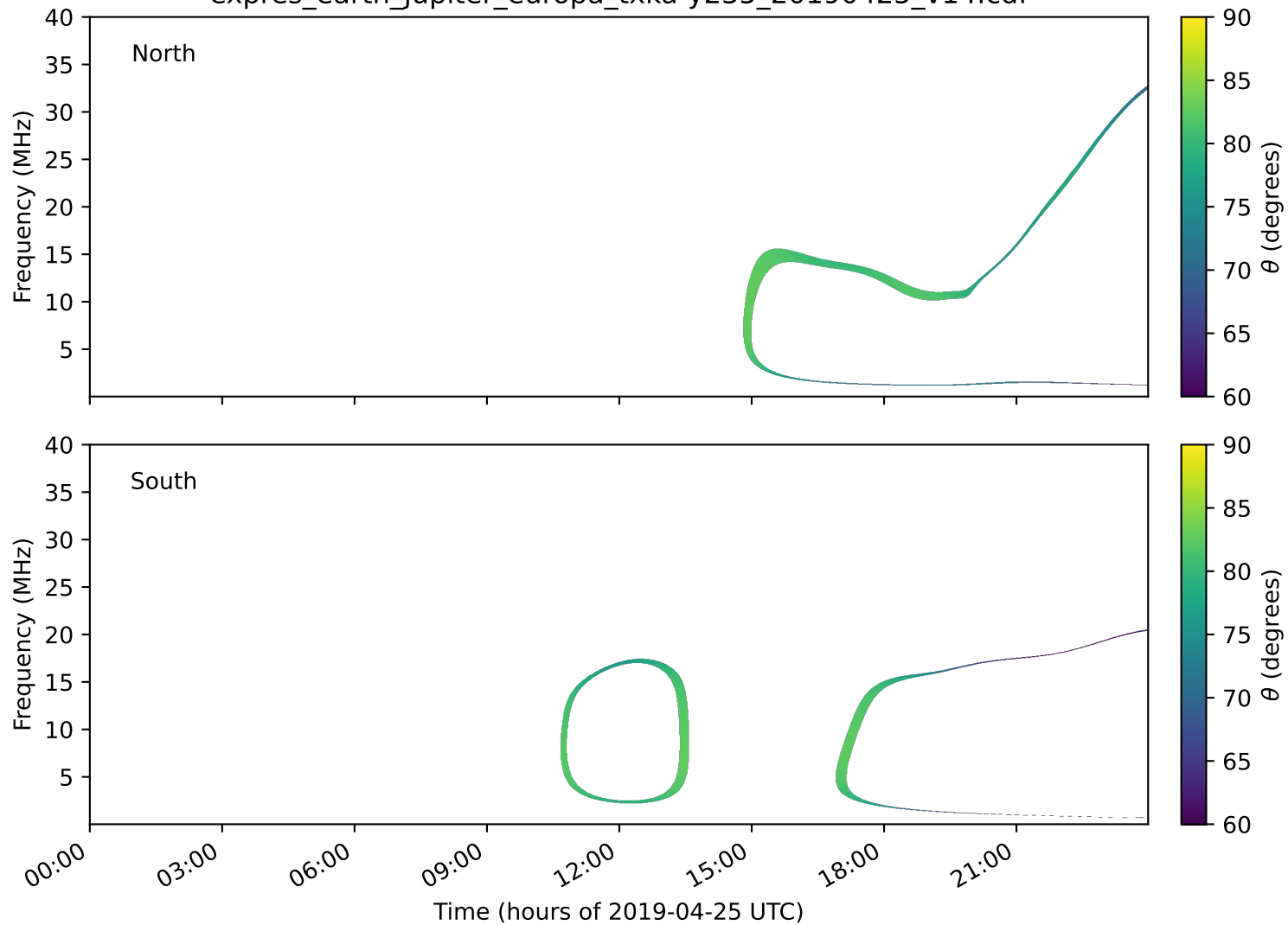
expres_earth_jupiter_europa_txka-y235_20190425_v14.cdf
