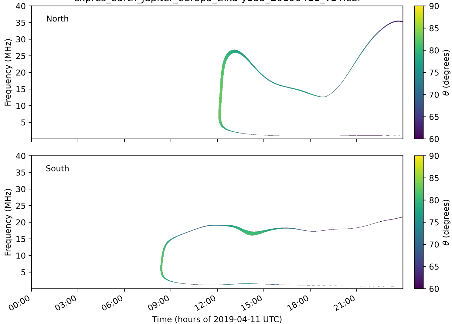
expres_earth_jupiter_europa_txka-y235_20190411_v14.cdf
