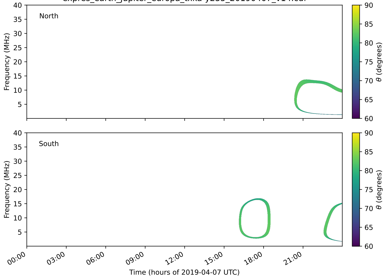
expres_earth_jupiter_europa_txka-y235_20190407_v14.cdf
