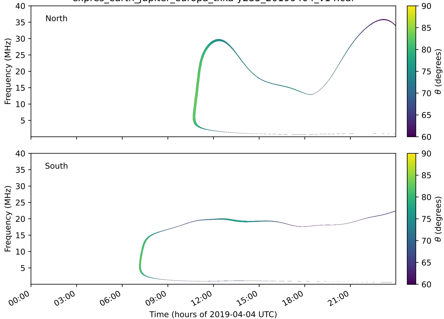
expres_earth_jupiter_europa_txka-y235_20190404_v14.cdf
