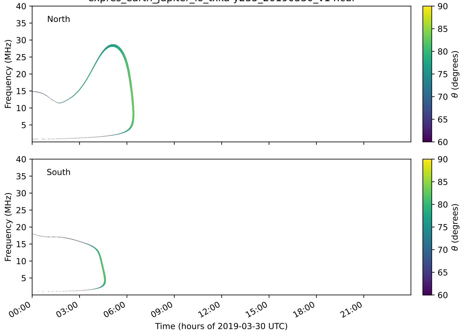
expres_earth_jupiter_io_txka-y235_20190330_v14.cdf
