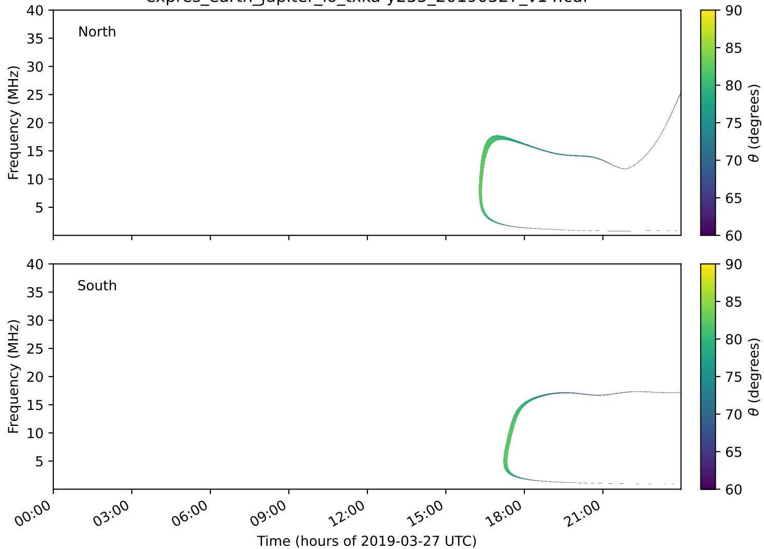
expres_earth_jupiter_io_txka-y235_20190327_v14.cdf
