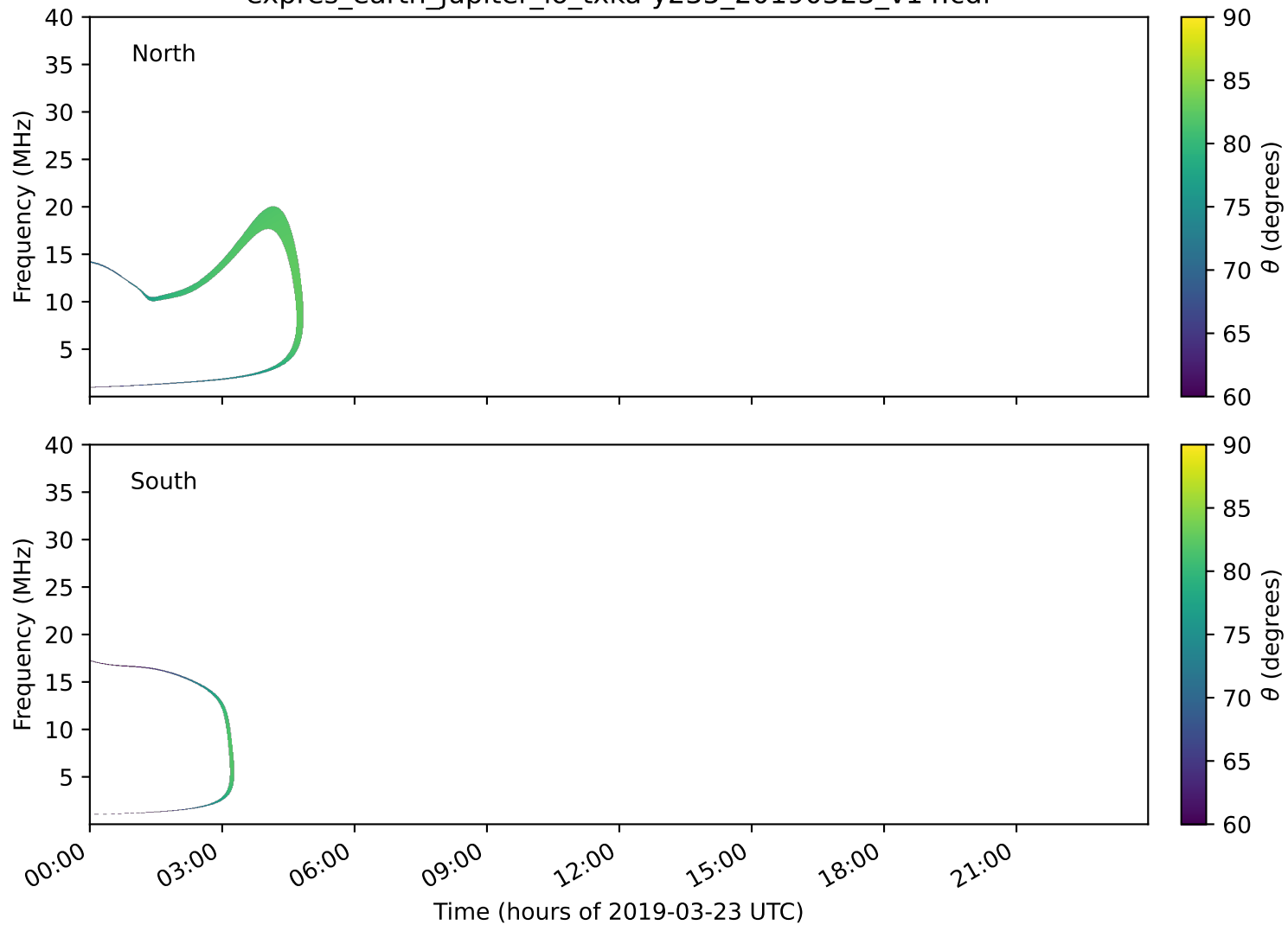
expres_earth_jupiter_io_txka-y235_20190323_v14.cdf
