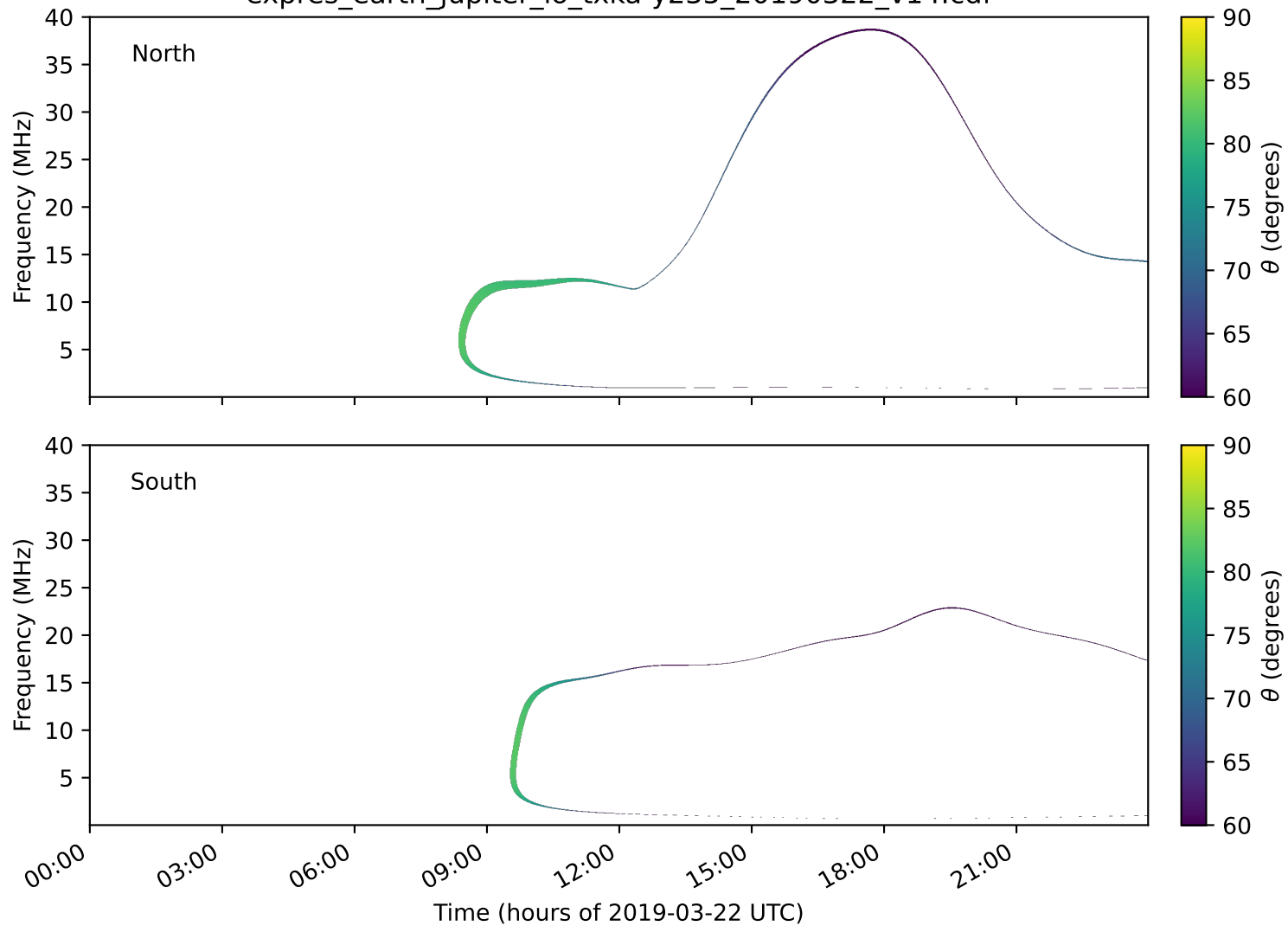
expres_earth_jupiter_io_txka-y235_20190322_v14.cdf
