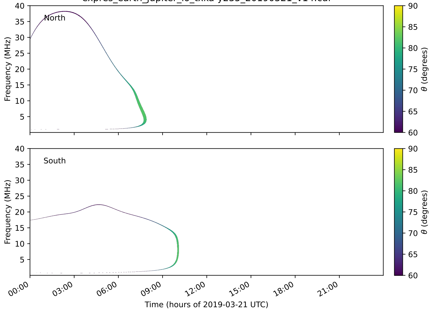
expres_earth_jupiter_io_txka-y235_20190321_v14.cdf
