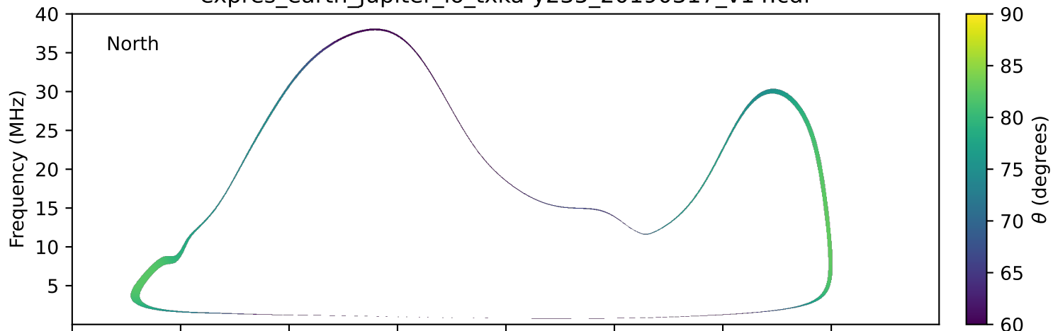
expres_earth_jupiter_io_txka-y235_20190317_v14.cdf
