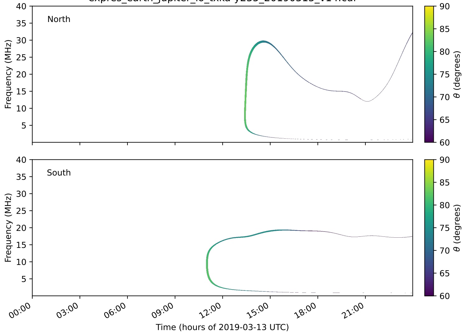
expres_earth_jupiter_io_txka-y235_20190313_v14.cdf
