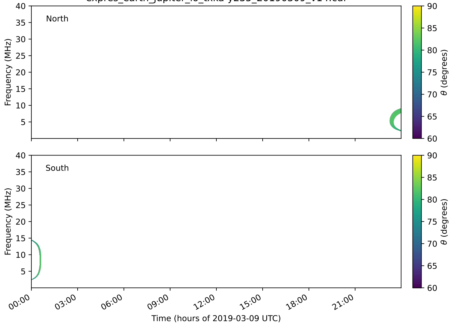
expres_earth_jupiter_io_txka-y235_20190309_v14.cdf
