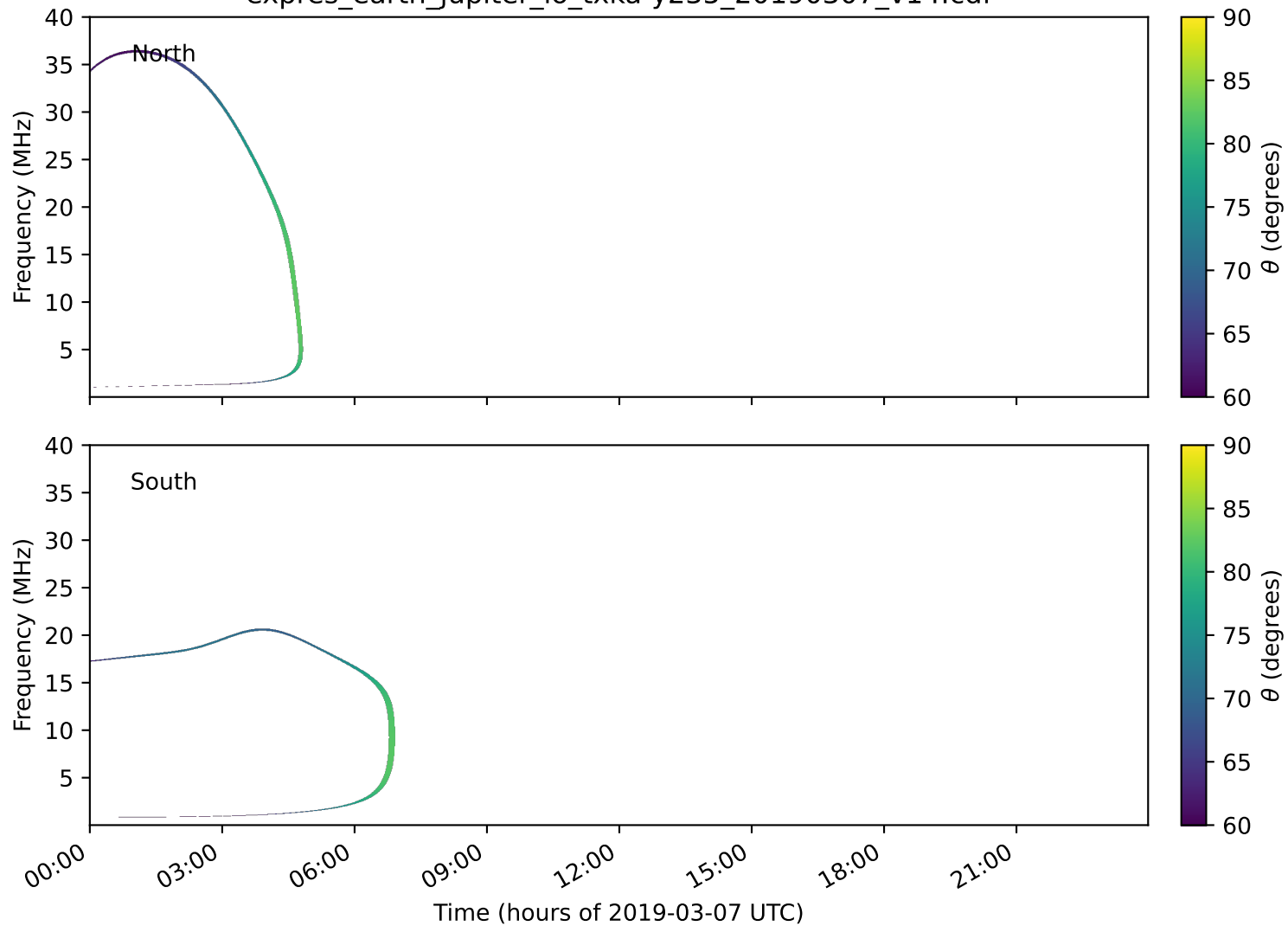
expres_earth_jupiter_io_txka-y235_20190307_v14.cdf
