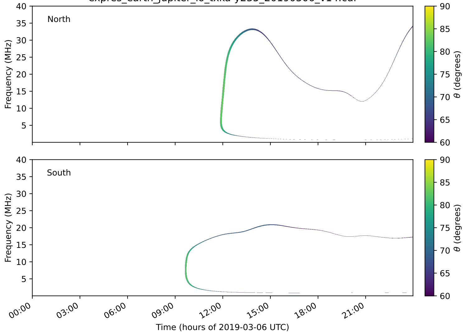
expres_earth_jupiter_io_txka-y235_20190306_v14.cdf
