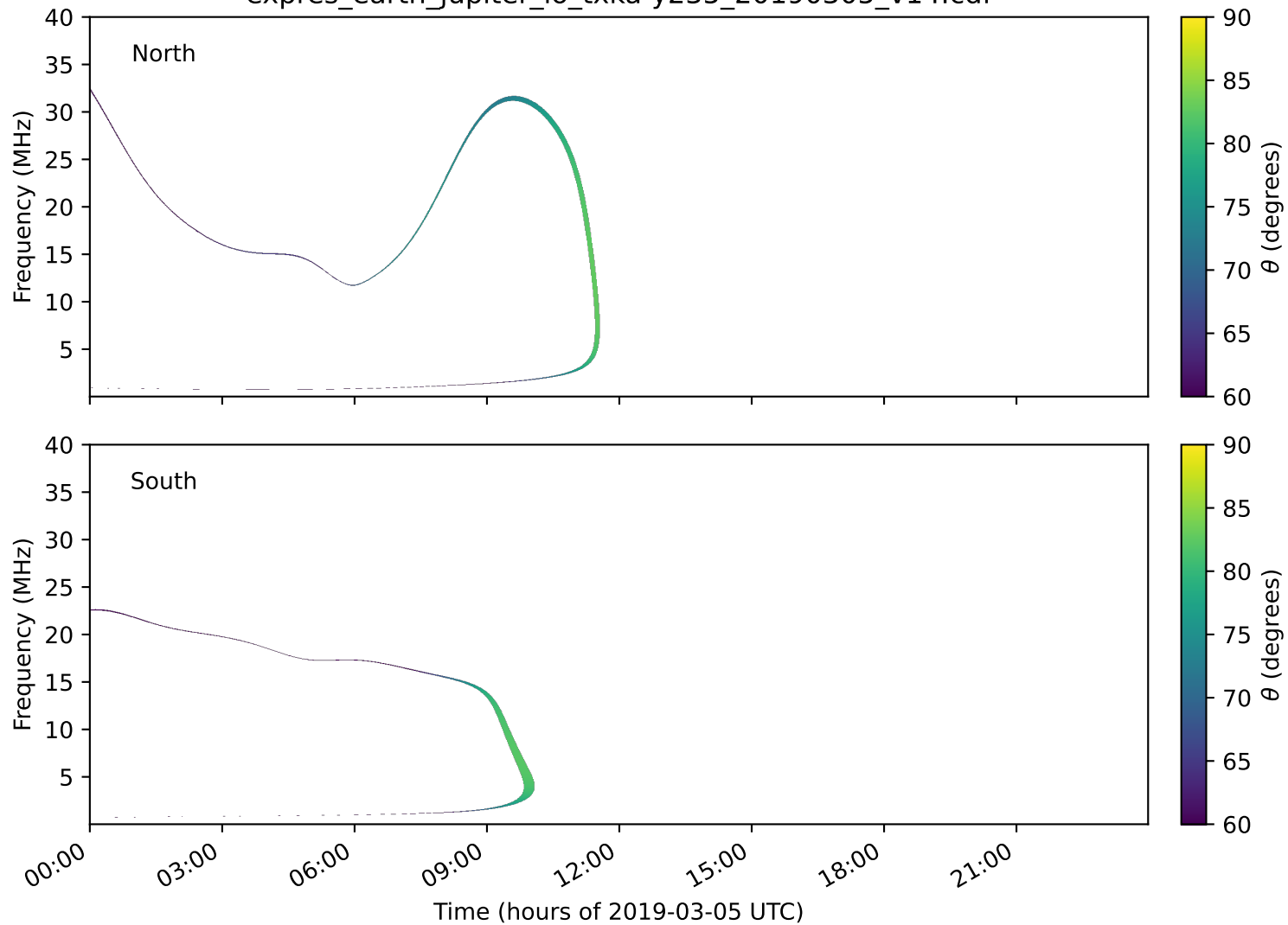
expres_earth_jupiter_io_txka-y235_20190305_v14.cdf
