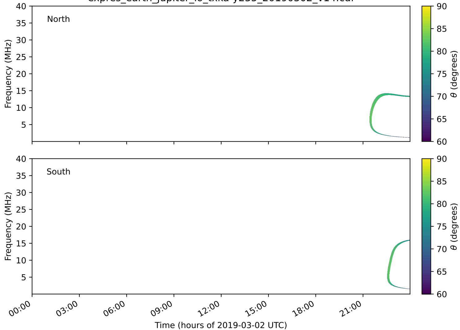
expres_earth_jupiter_io_txka-y235_20190302_v14.cdf
