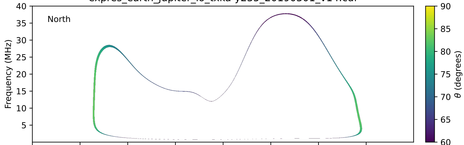
expres_earth_jupiter_io_txka-y235_20190301_v14.cdf
