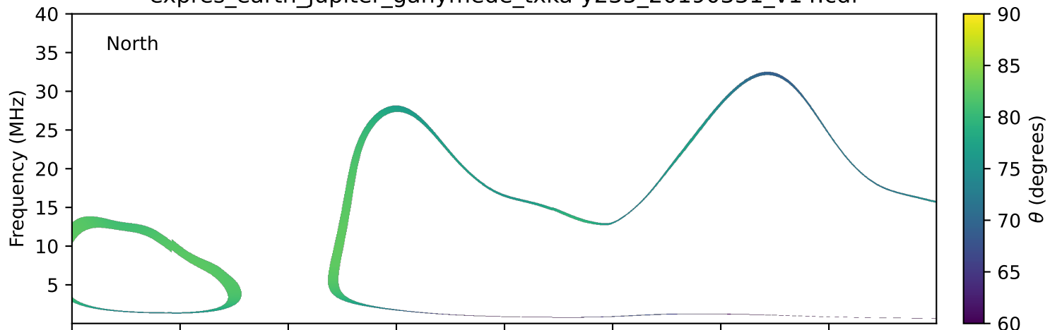
expres_earth_jupiter_ganymede_txka-y235_20190331_v14.cdf
