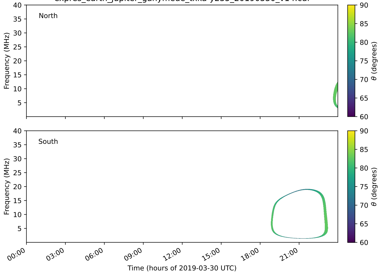
expres_earth_jupiter_ganymede_txka-y235_20190330_v14.cdf
