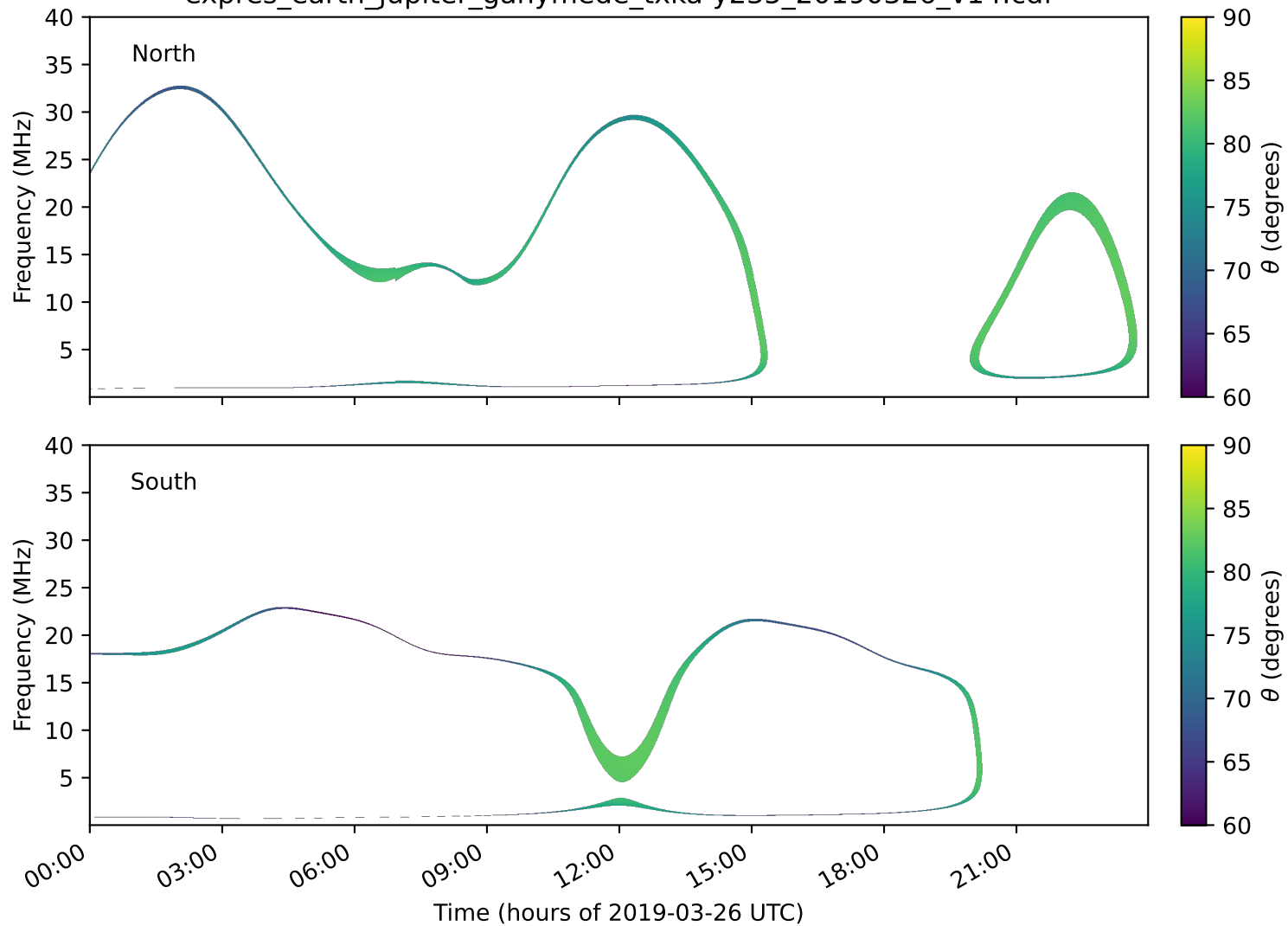
expres_earth_jupiter_ganymede_txka-y235_20190326_v14.cdf
