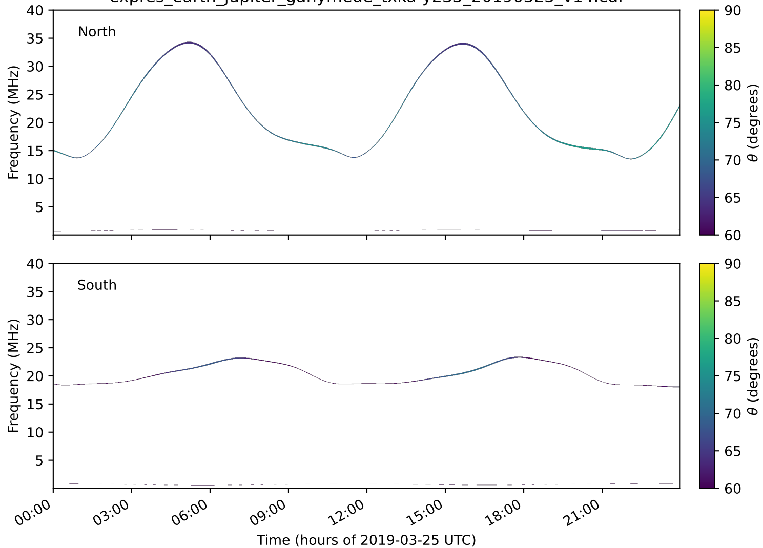
expres_earth_jupiter_ganymede_txka-y235_20190325_v14.cdf
