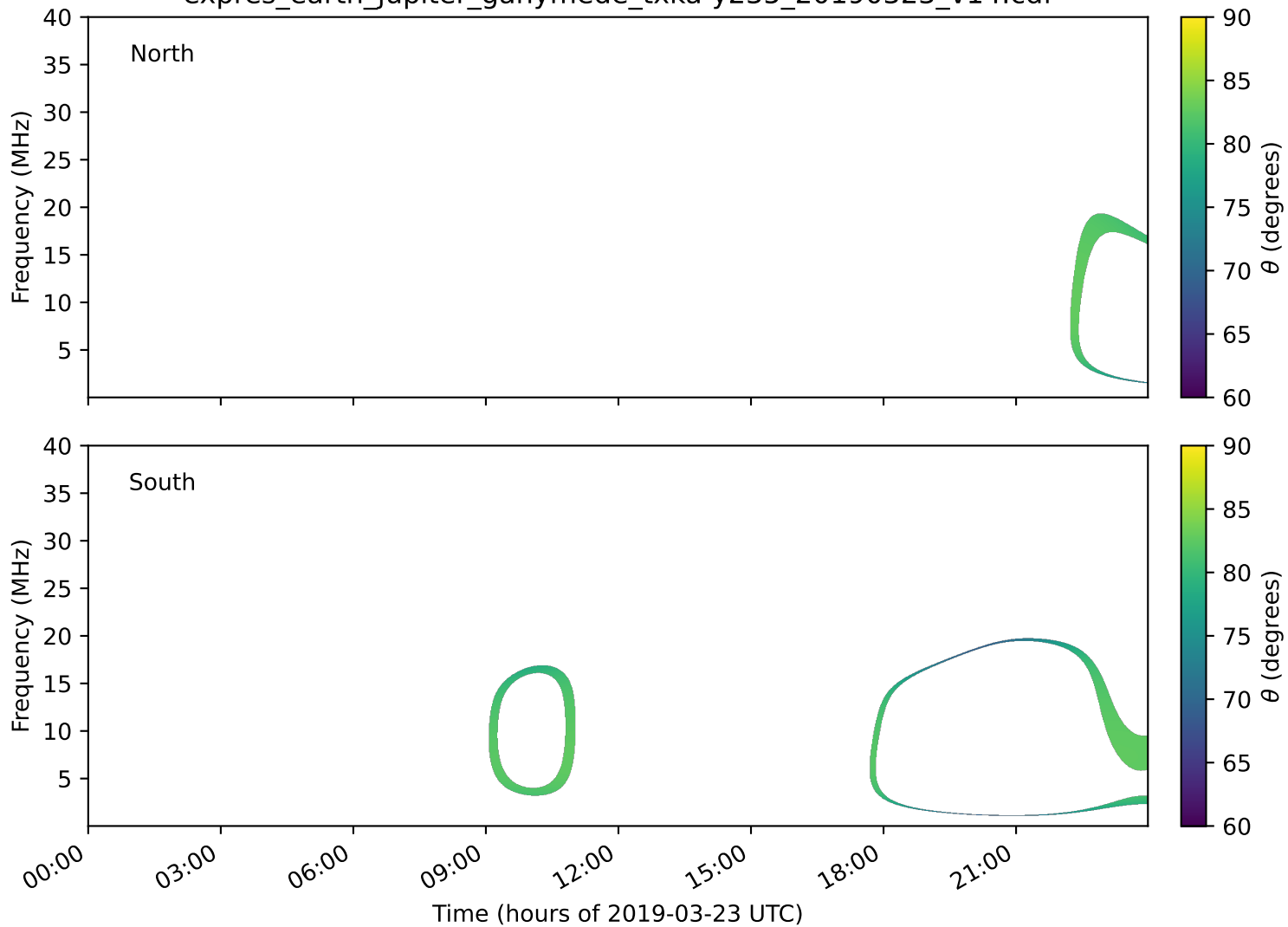
expres_earth_jupiter_ganymede_txka-y235_20190323_v14.cdf
