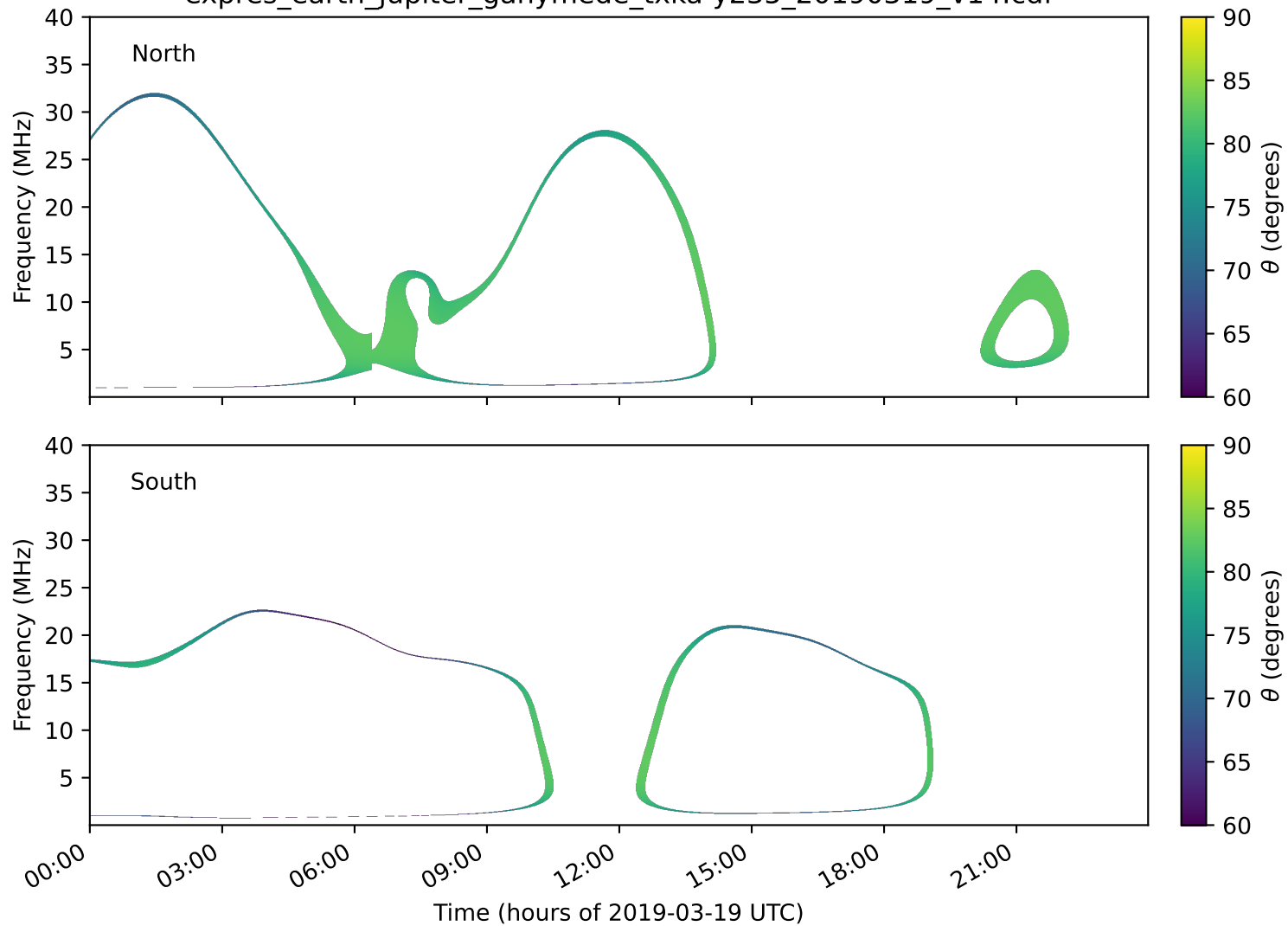
expres_earth_jupiter_ganymede_txka-y235_20190319_v14.cdf
