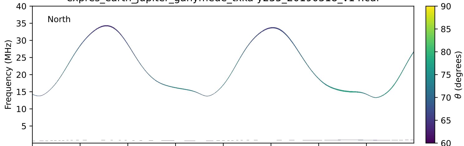
expres_earth_jupiter_ganymede_txka-y235_20190318_v14.cdf
