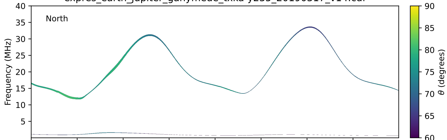
expres_earth_jupiter_ganymede_txka-y235_20190317_v14.cdf
