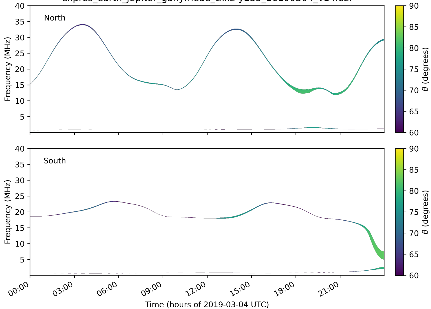
expres_earth_jupiter_ganymede_txka-y235_20190304_v14.cdf
