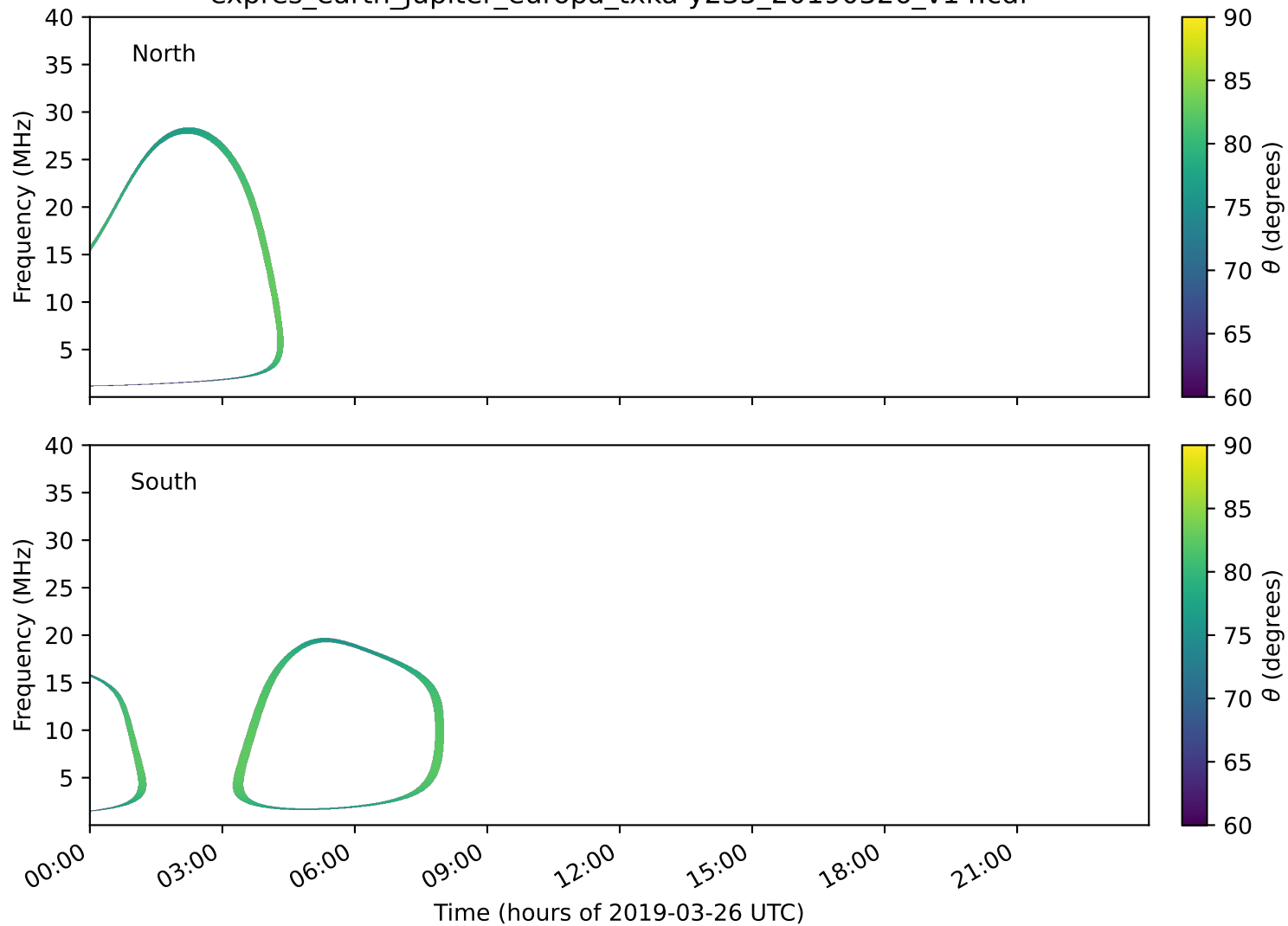
expres_earth_jupiter_europa_txka-y235_20190326_v14.cdf
