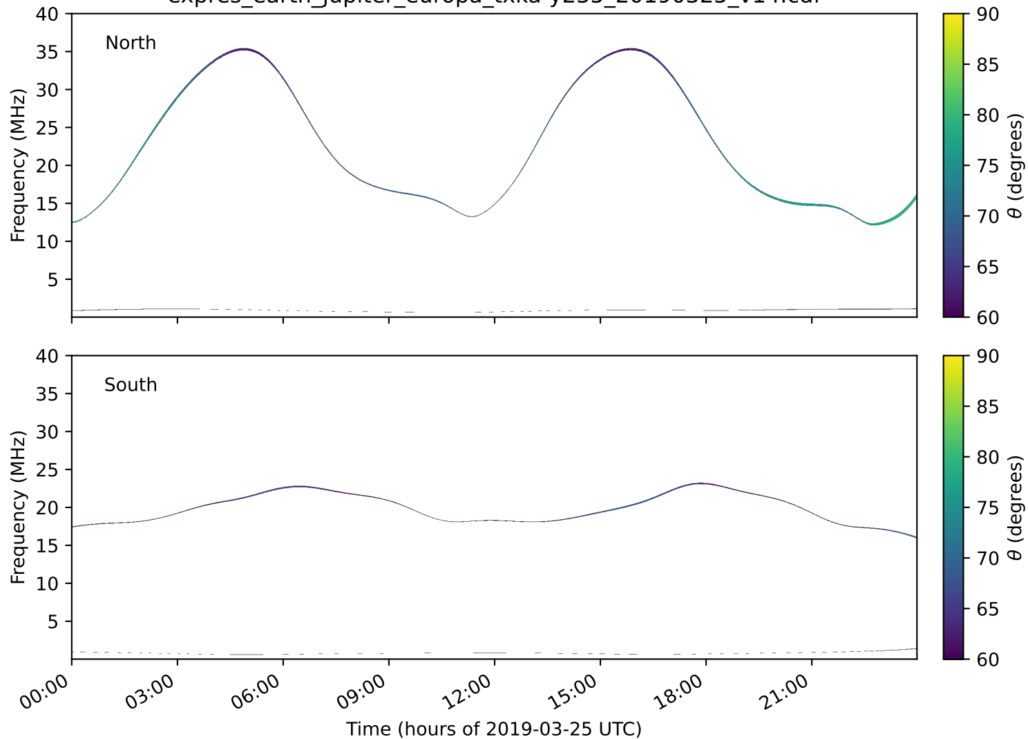
expres_earth_jupiter_europa_txka-y235_20190325_v14.cdf
