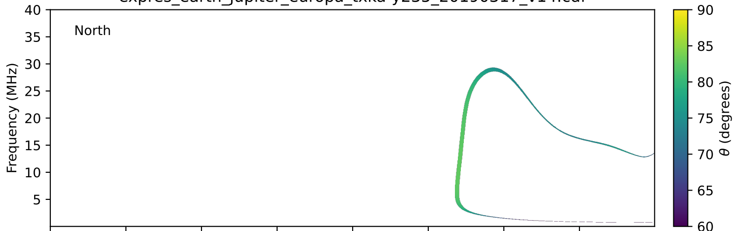
expres_earth_jupiter_europa_txka-y235_20190317_v14.cdf
