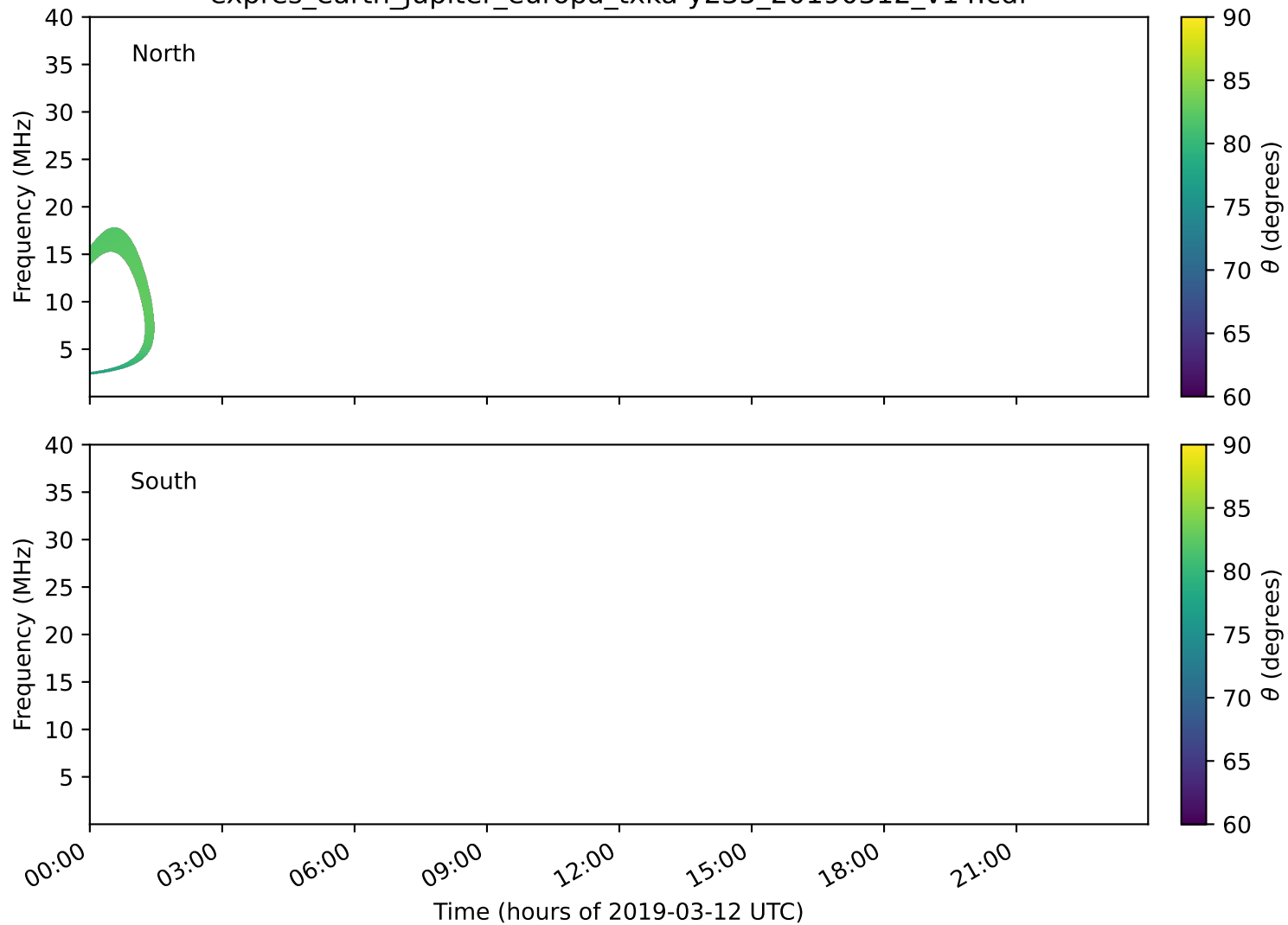
expres_earth_jupiter_europa_txka-y235_20190312_v14.cdf
