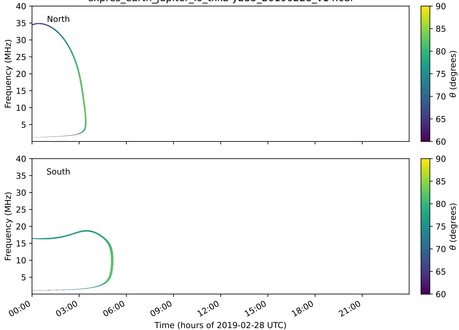
expres_earth_jupiter_io_txka-y235_20190228_v14.cdf
