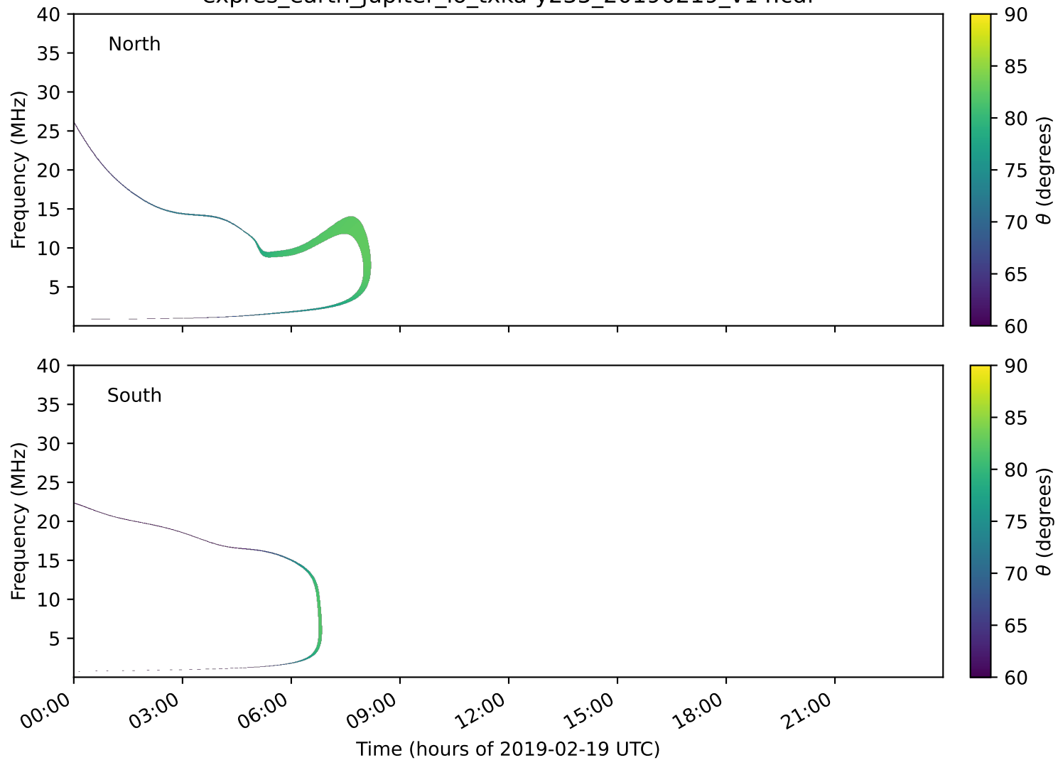
expres_earth_jupiter_io_txka-y235_20190219_v14.cdf
