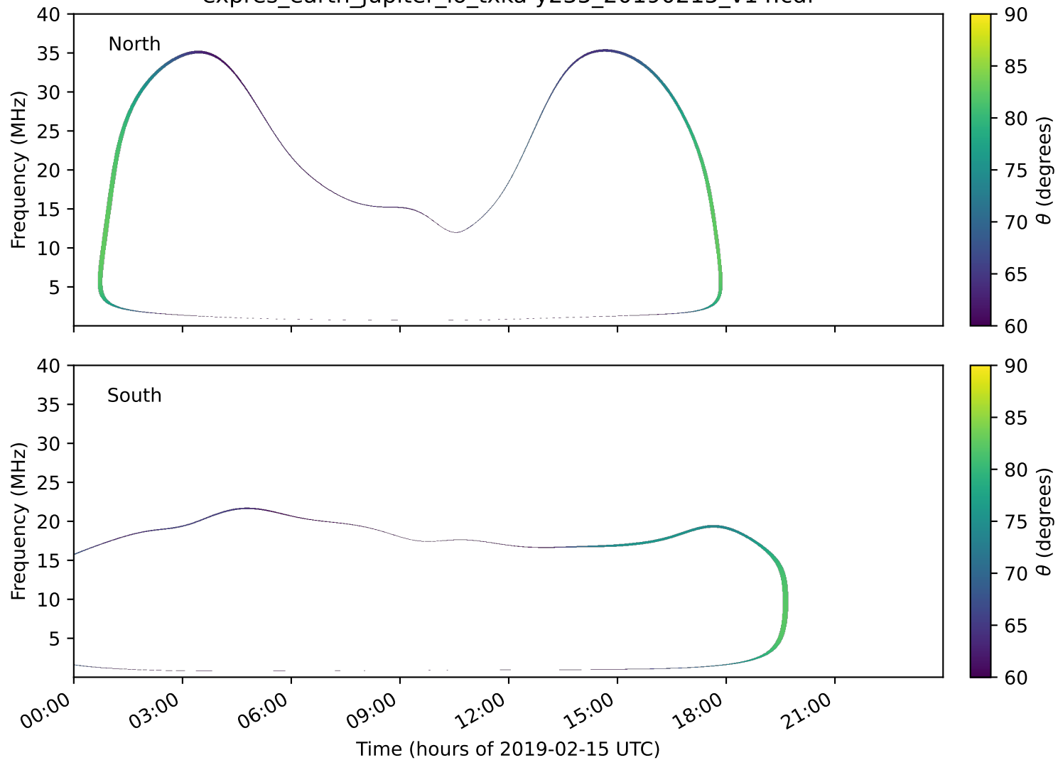
expres_earth_jupiter_io_txka-y235_20190215_v14.cdf
