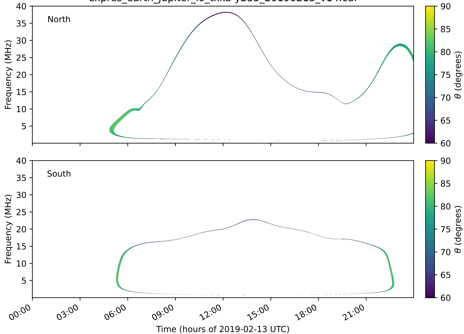
expres_earth_jupiter_io_txka-y235_20190213_v14.cdf
