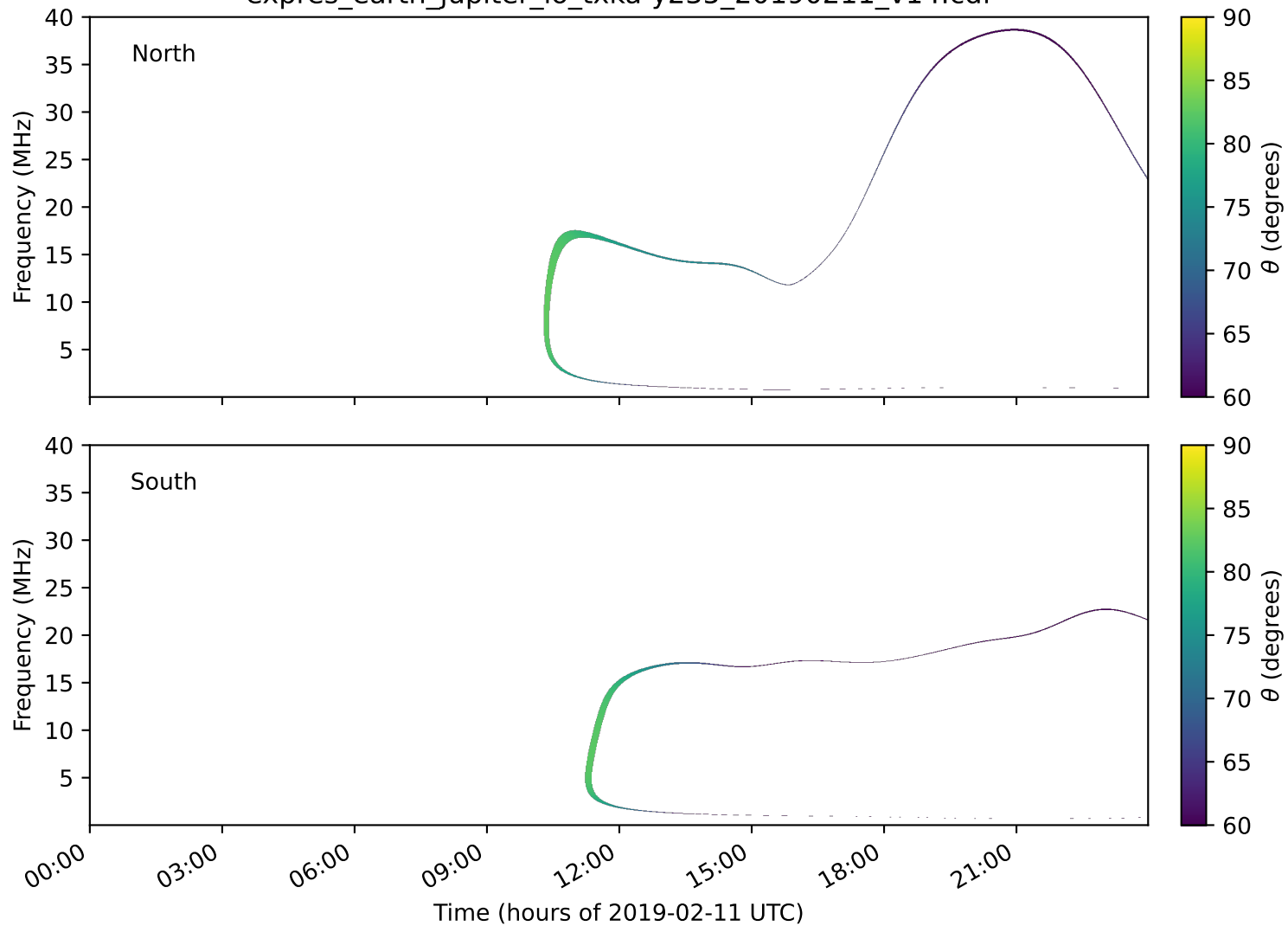
expres_earth_jupiter_io_txka-y235_20190211_v14.cdf
